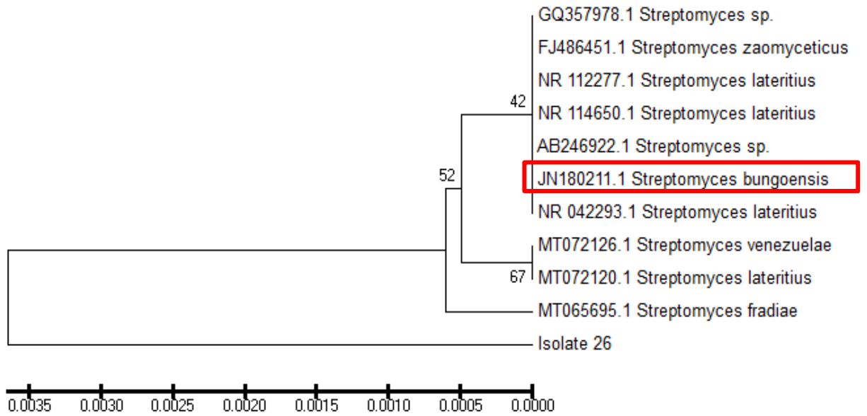
Figure 6: Phylogenetic tree of the nucleotide sequences of the PCR product of 16S rRNA gene amplified from the DNA of Streptomyces strain BF26 and universal bacterial strains from BLAST.
